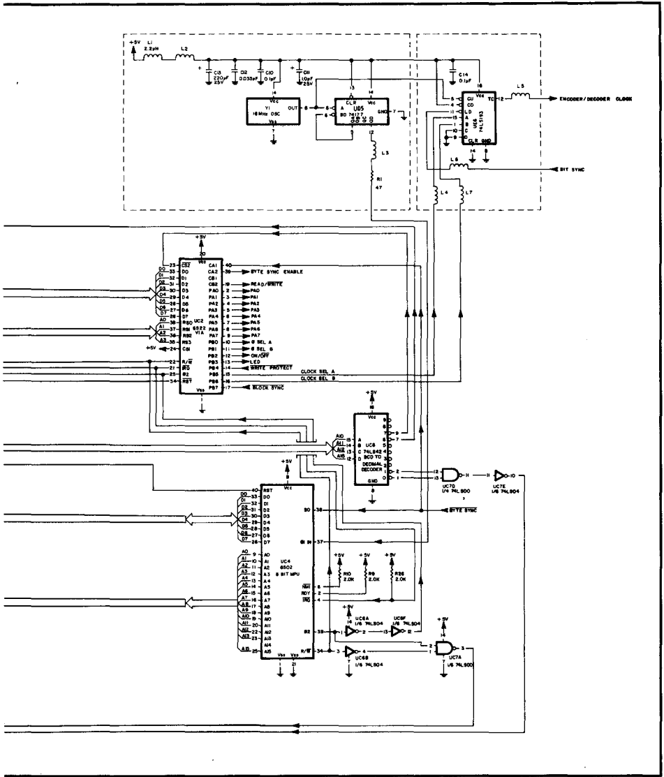
schematic, Model 1542.
